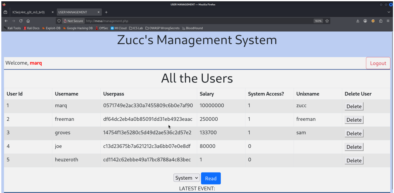
Figure 66: Accessing the management system as user marq
